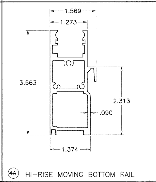
4 STD. MOVING BOTTOM RAIL
